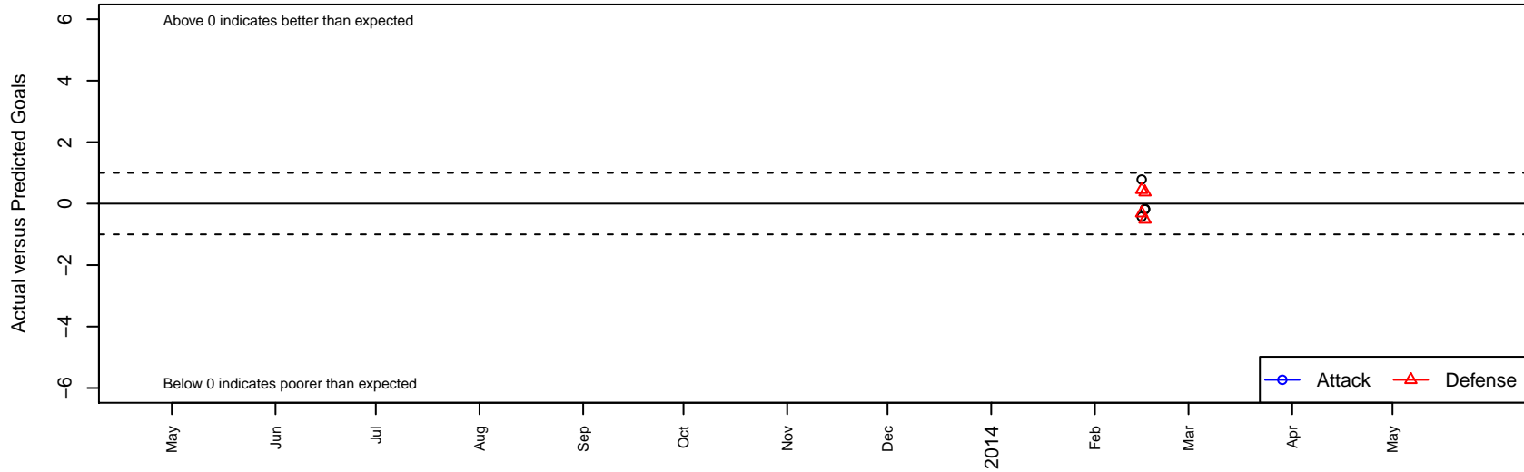
United SA Elite Black G01 Dots are actual minus expected GF (blue circles) and GA (red triangles). Blue line is smoothed change in attack strength. Red is smoothed change in defense strength.
